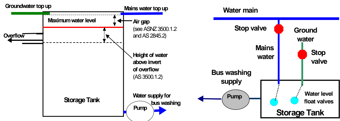
Figure 2.19: Configuration of the mains water and groundwater top up of the bus washing storage tank.
